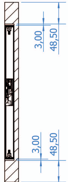
SECTION B-B
